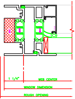
430 JAMB 325 CASEMENT IN 4-BAR ARMS
