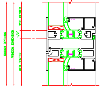
531 MEETING RAIL 325 FIXED \ CASEMENT IN BUTT HINGES
