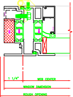
432 JAMB 325 CASEMENT IN BUTT HINGES
